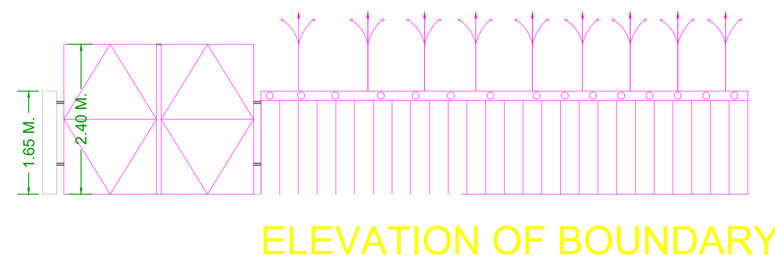
FRONT ELEVATION
