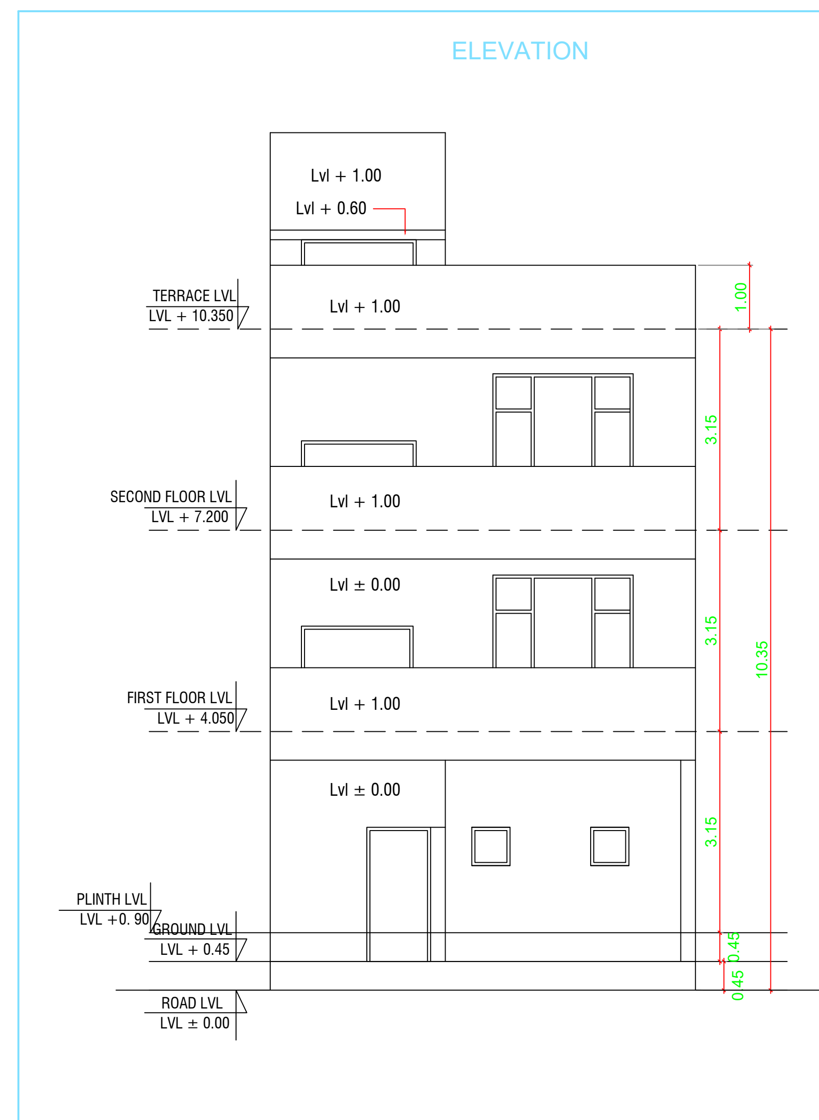
FRONT ELEVATION
