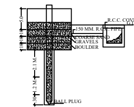
SECTION DETAIL OF HARVESTING TANK (SCALE : N.T.S.)
