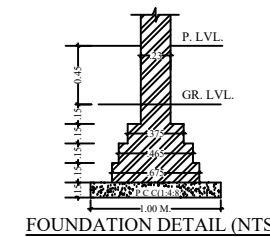
FOUNDATION DETAIL (NTS.)
